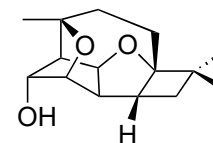
(+)-Punctaporonin U
