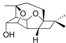
(+)-Punctaporonin U
